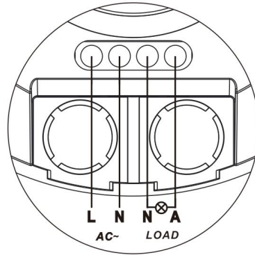
The wires come in and out from the side
